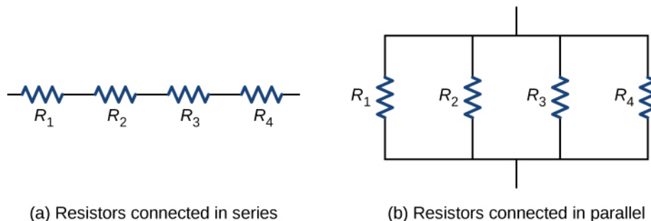
Figure 10.11 (a) For a series connection of resistors, the current is the same in each resistor. (b) For a parallel connection of resistors, the voltage is the same across each resistor.
