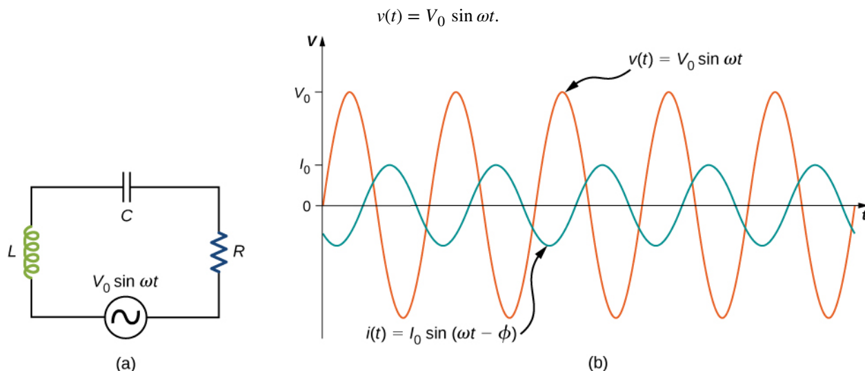
Figure 15.11 (a) An RLC series circuit. (b) A comparison of the generator output voltage and the current. The value of the phase difference \phi depends on the values of R , C , and L .
